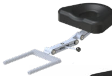
10-230-Mdbl C-C: 171,5 mm ø: 18 mm Length: 170 mm
